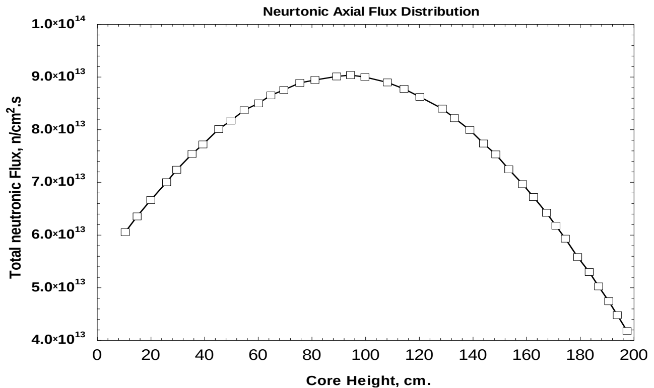
Fig. 12. Axial total flux distribution for HTR-10 versus core height
