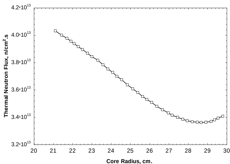
Fig. 6. Radial thermal flux distribution for HTR-10 versus core radius
