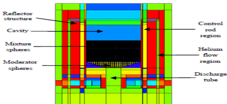
Fig. 2. MCNP6 Model of HTR-10 (Vertical Cross Section).
