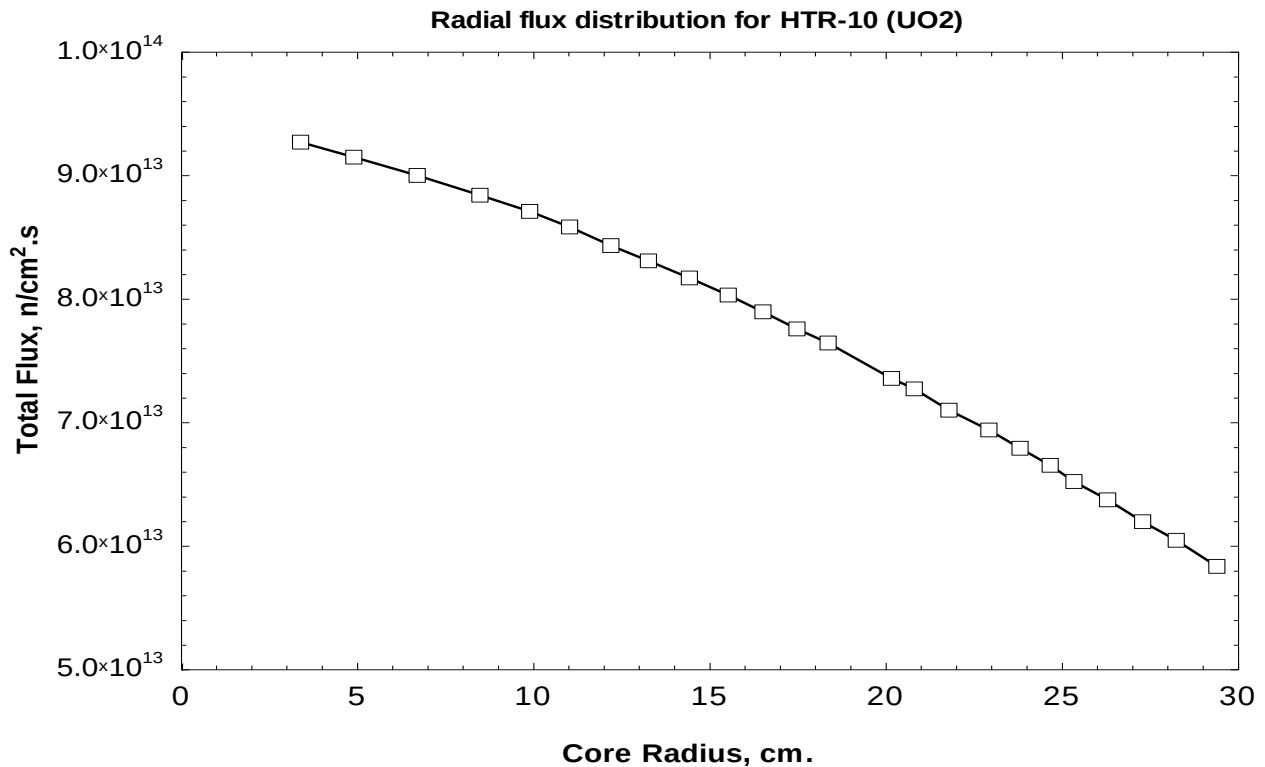
Fig. 8. Radial total flux distribution for HTR-10 versus core radius
