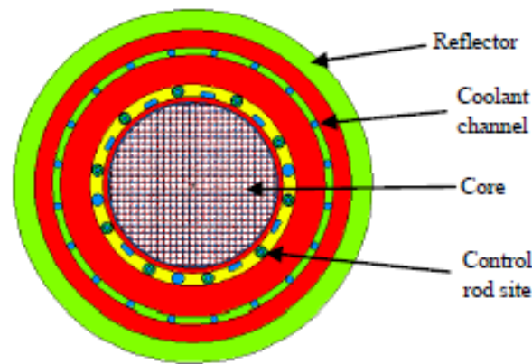
Fig. 3. MCNP6 Model of HTR-10 (Horizontal Cross Section).
