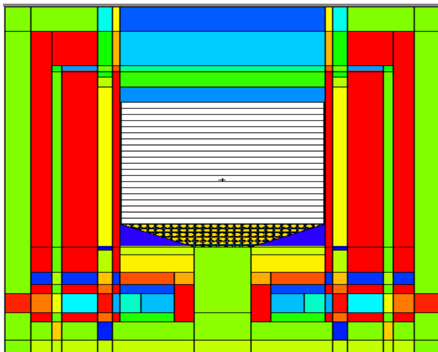
Fig. 10. Axial zones for HTR-reactor
