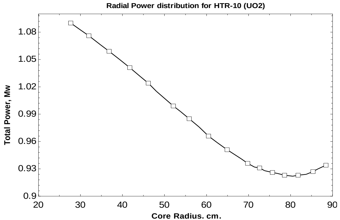
Fig. 9. Radial total power distribution for HTR-10 versus core radius
