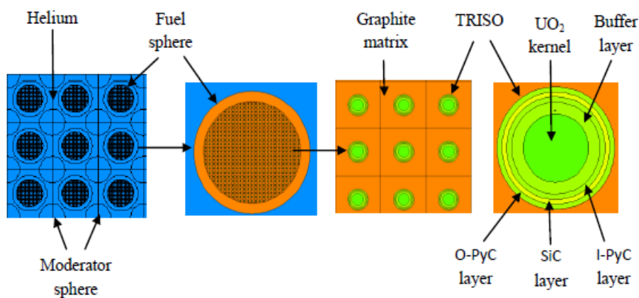
Fig. 4. Pebble-bed and moderator ball in a BCC lattice and TRISO in the reactor core model.
