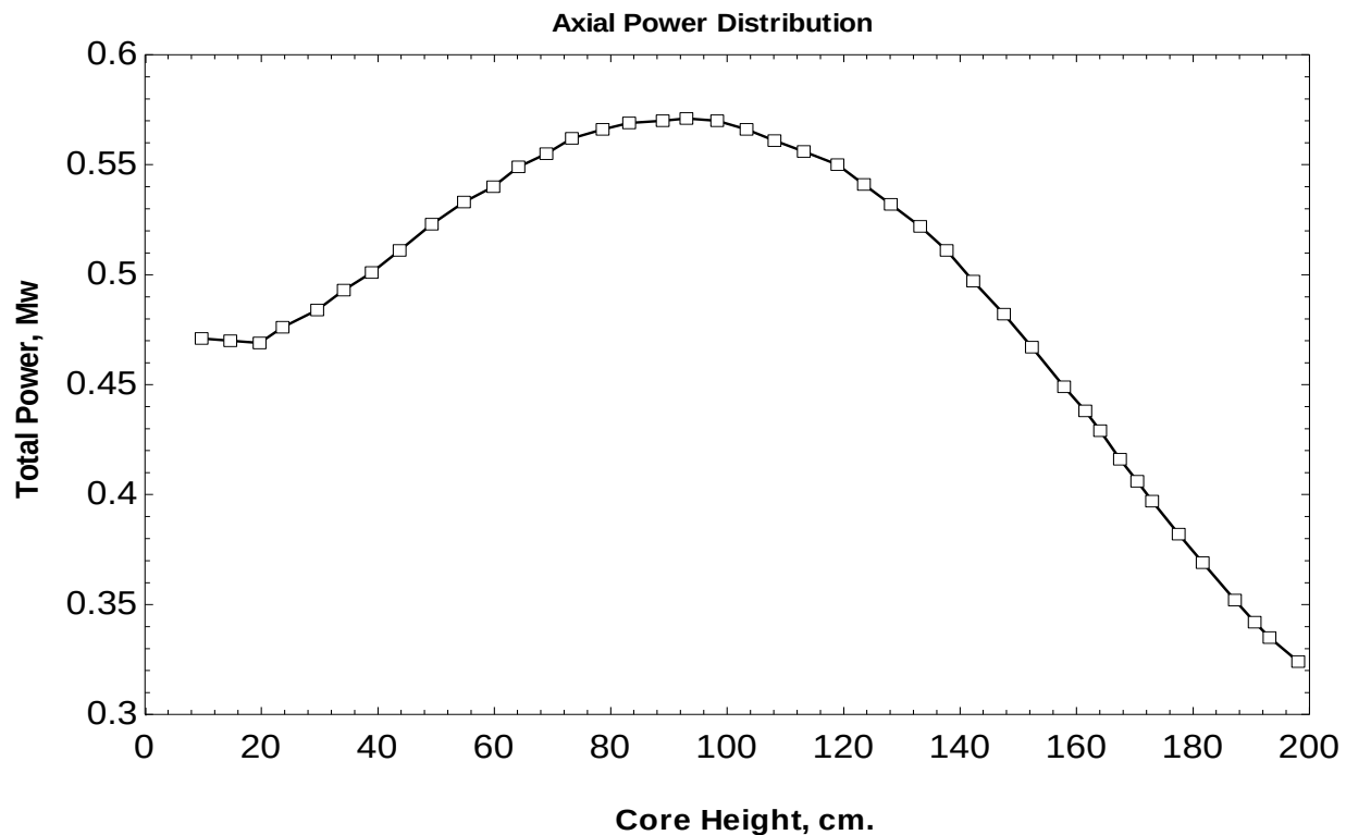
Fig. 13. Axial total power distribution for HTR-10 versus core height
