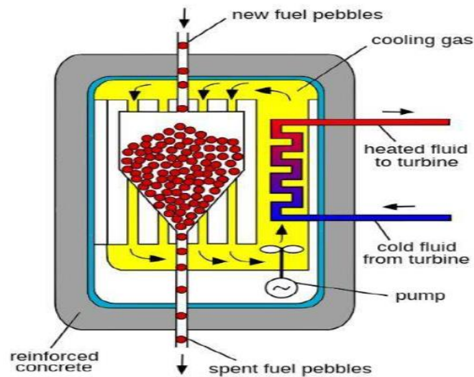
Fig. 1: Schematic of the pebble bed reactor [4].
