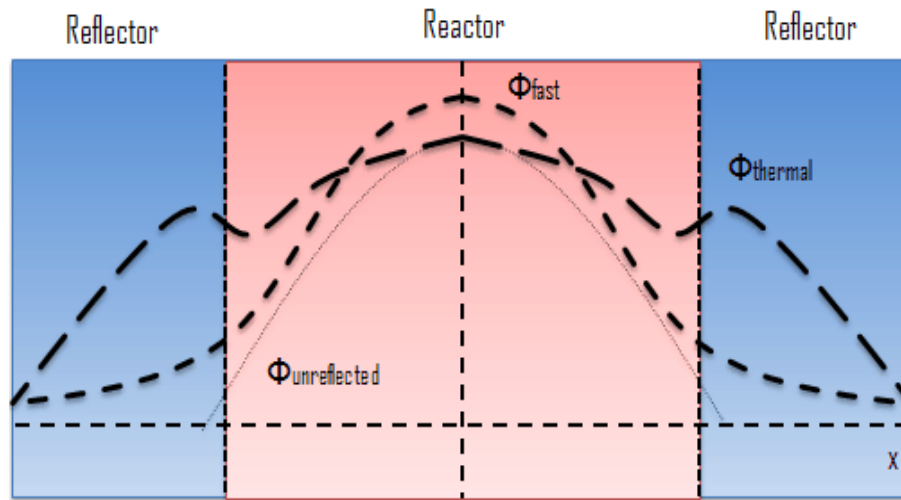
Fig. 7. Effect of reflection in the thermal reactor
